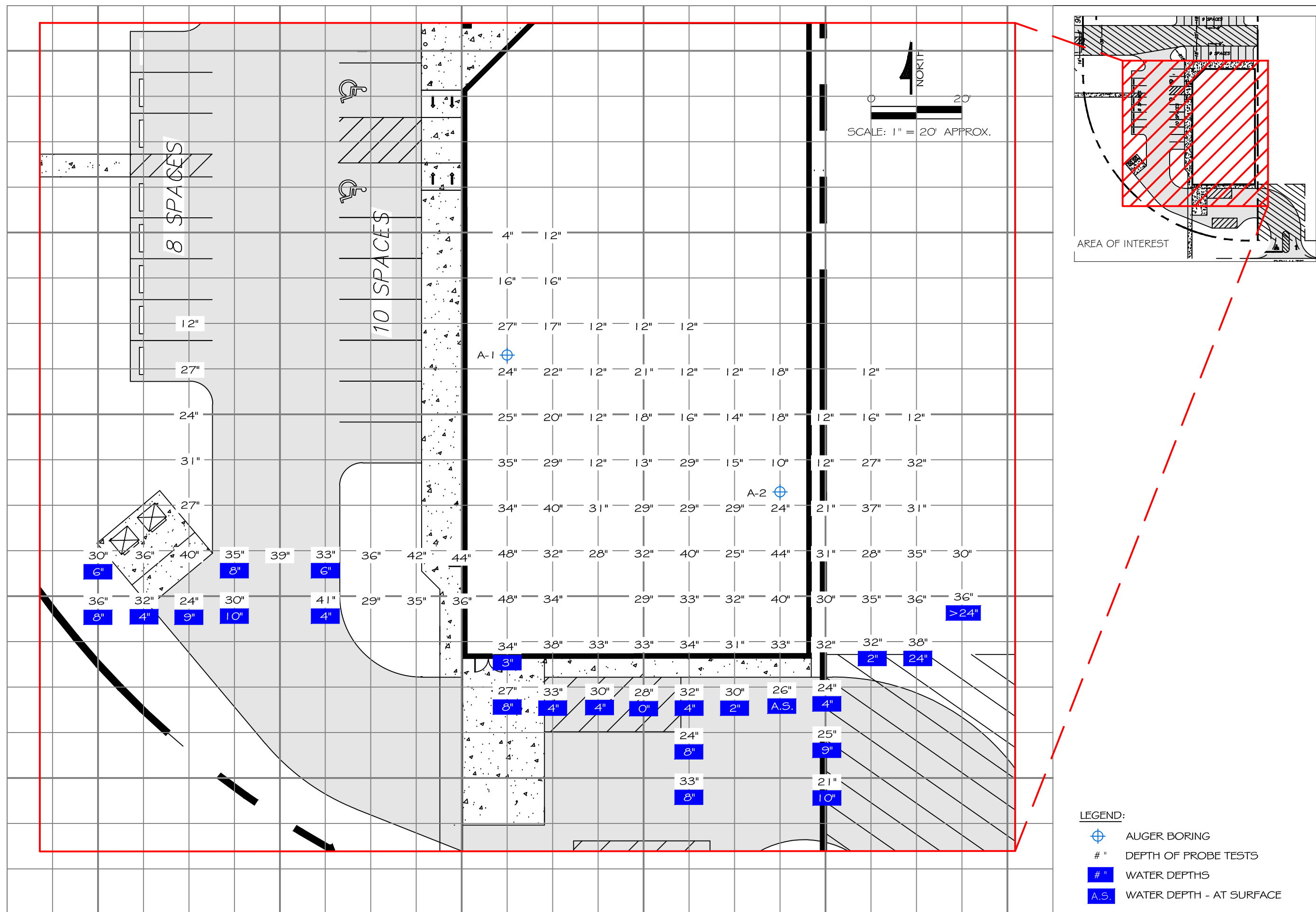
SITE PLAN APPROXIMATE SHOWING LOCATIONS OF MUCK PROBE TESTS AND WATER DEPTHS
