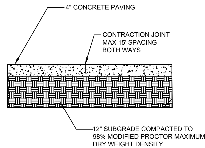
CONCRETE PAVING SECTION NTS
