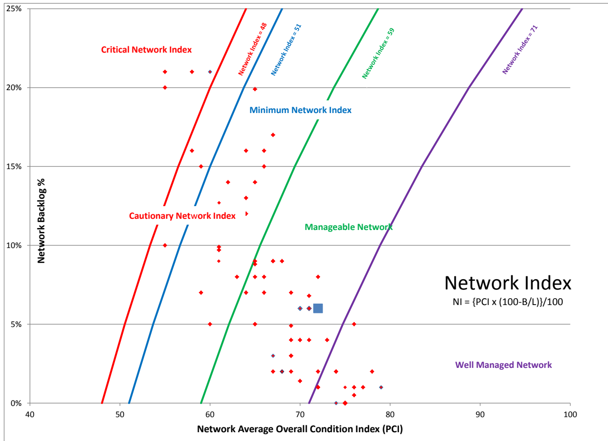
Figure 24 – Network Index
